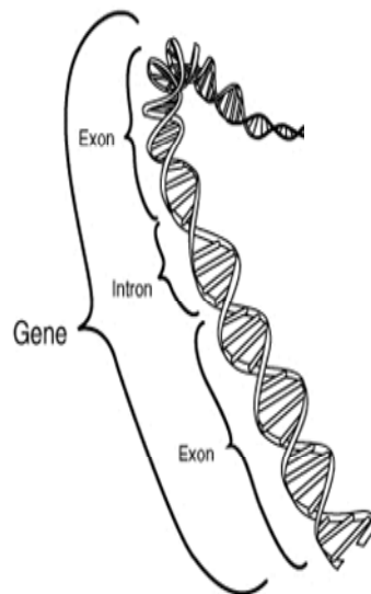
Figure 2. Gene
