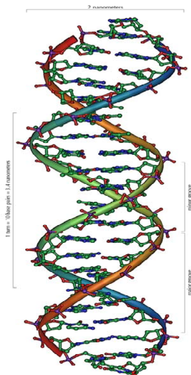
Figure 1. Deoxyribonucleic acid
